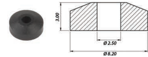
Conta Şamandıra Vana Pim Gasket for Multivalve Pin
